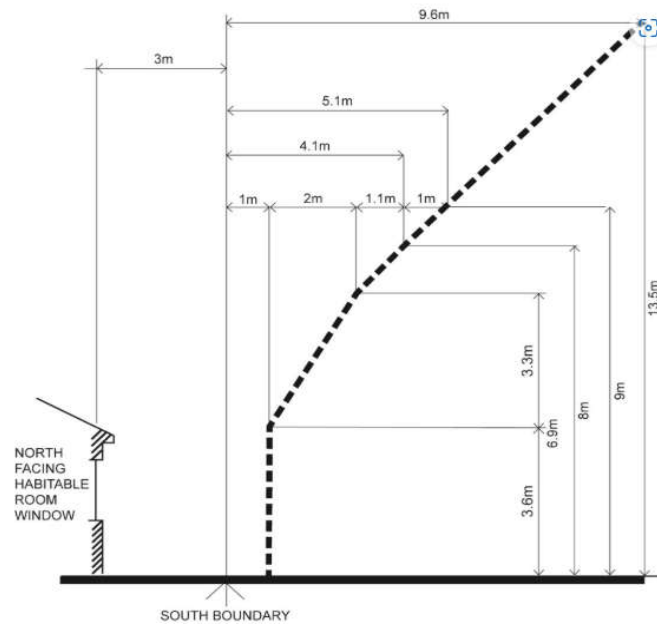
Diagram B4-2.2 North-facing windows
