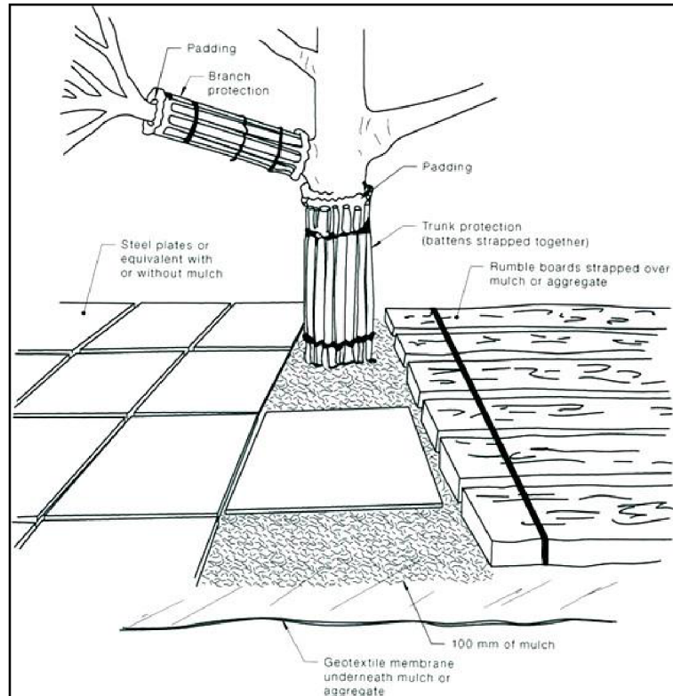
Ground protection examples
