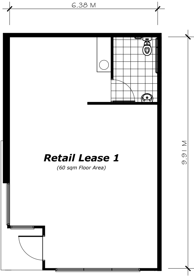
GRAHAM WALK
