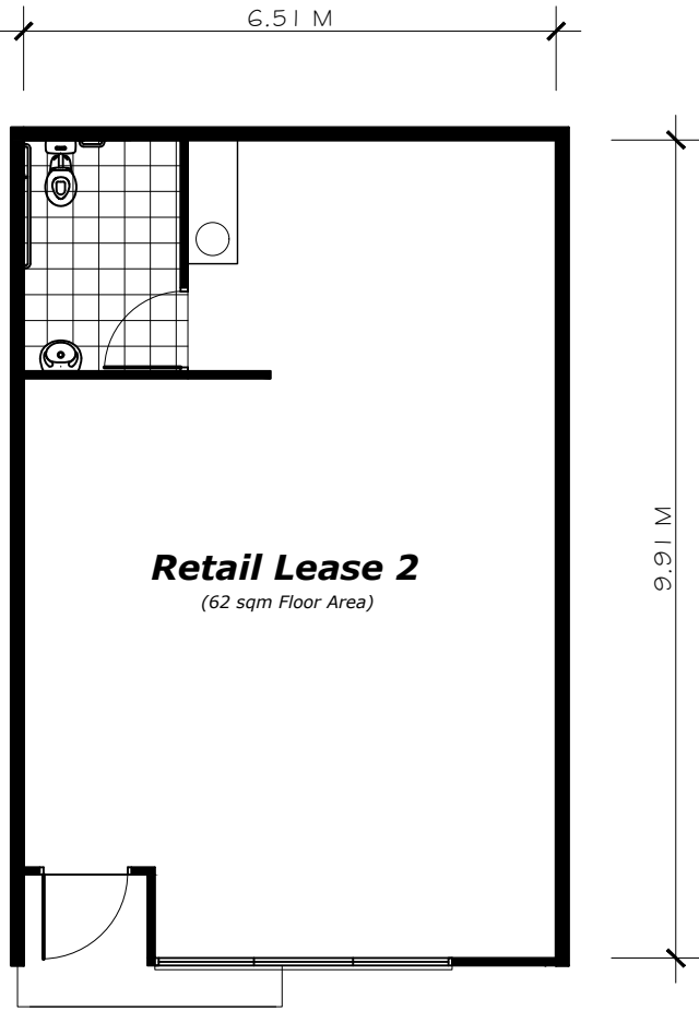
GRAHAM WALK
