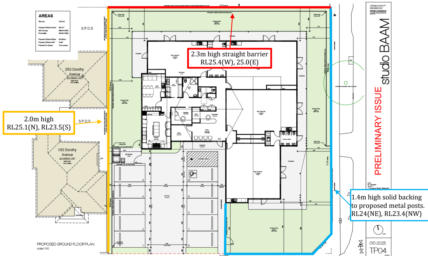
Figure 3: Acoustic barrier markup
