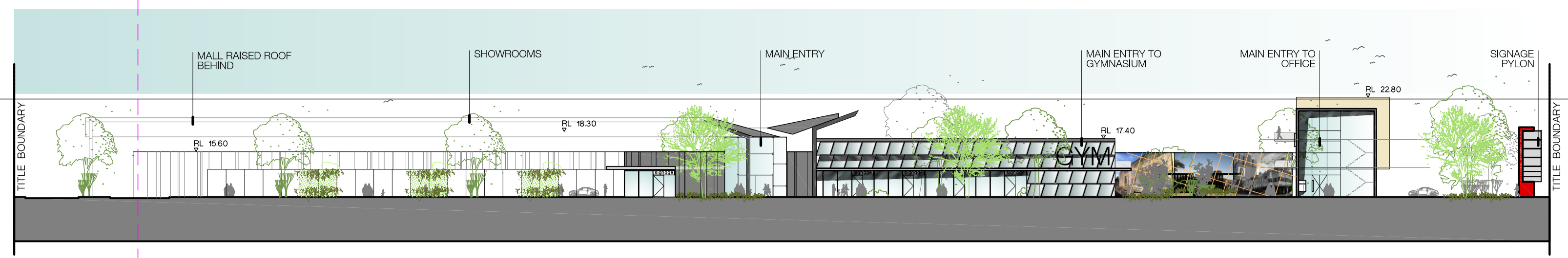
e1 TP-401 Western Elevation
