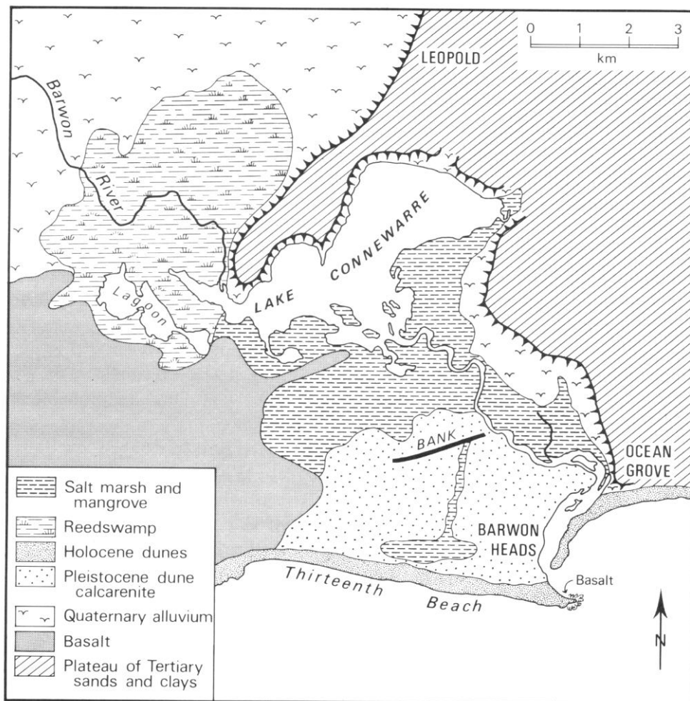
Figure 1: Simplified geology of the Lake Connewarre Complex (Bird 1993).
