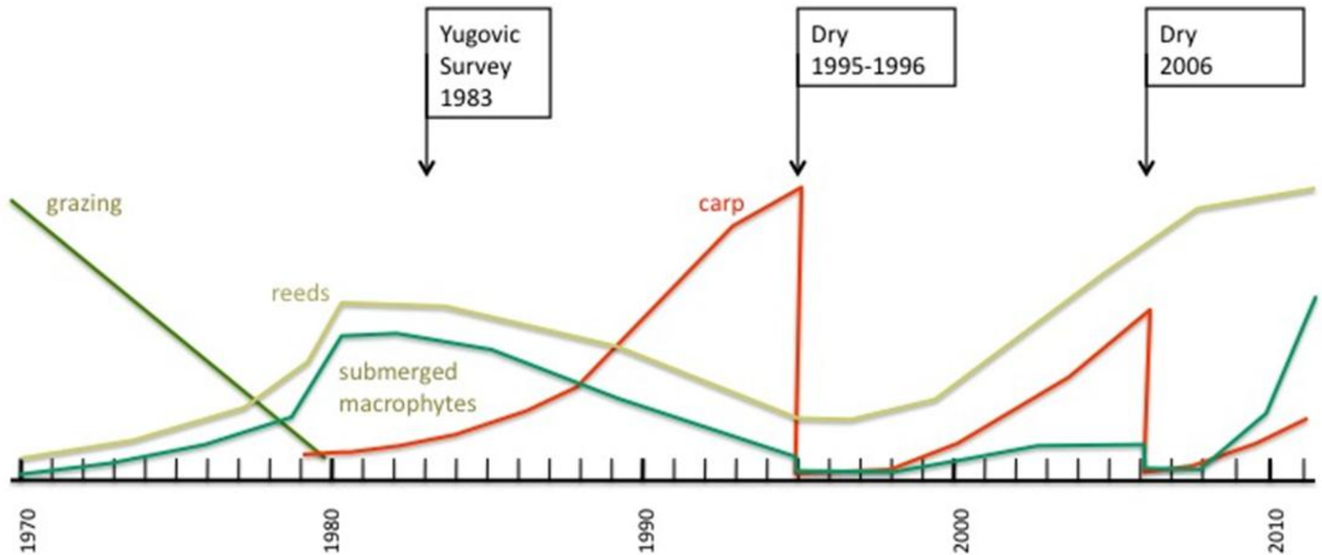
Figure 5: An overview of changes in reed and macrophyte cover, and relative carp populations in Reedy Lake since 1970. Carp were first recorded in the lower Barwon River in 1979, and Reedy Lake was subsequently dried in 1995/96 and 2006 to reduce carp populations in the lake. Grazing by cattle in Reedy Lake was curtailed and finally stopped during the 1970's.
