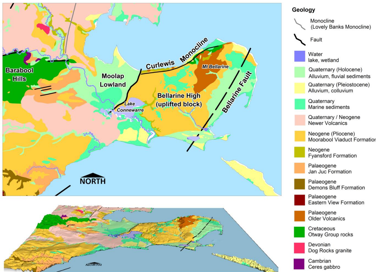
Figure 2: Geology and regional landform.
