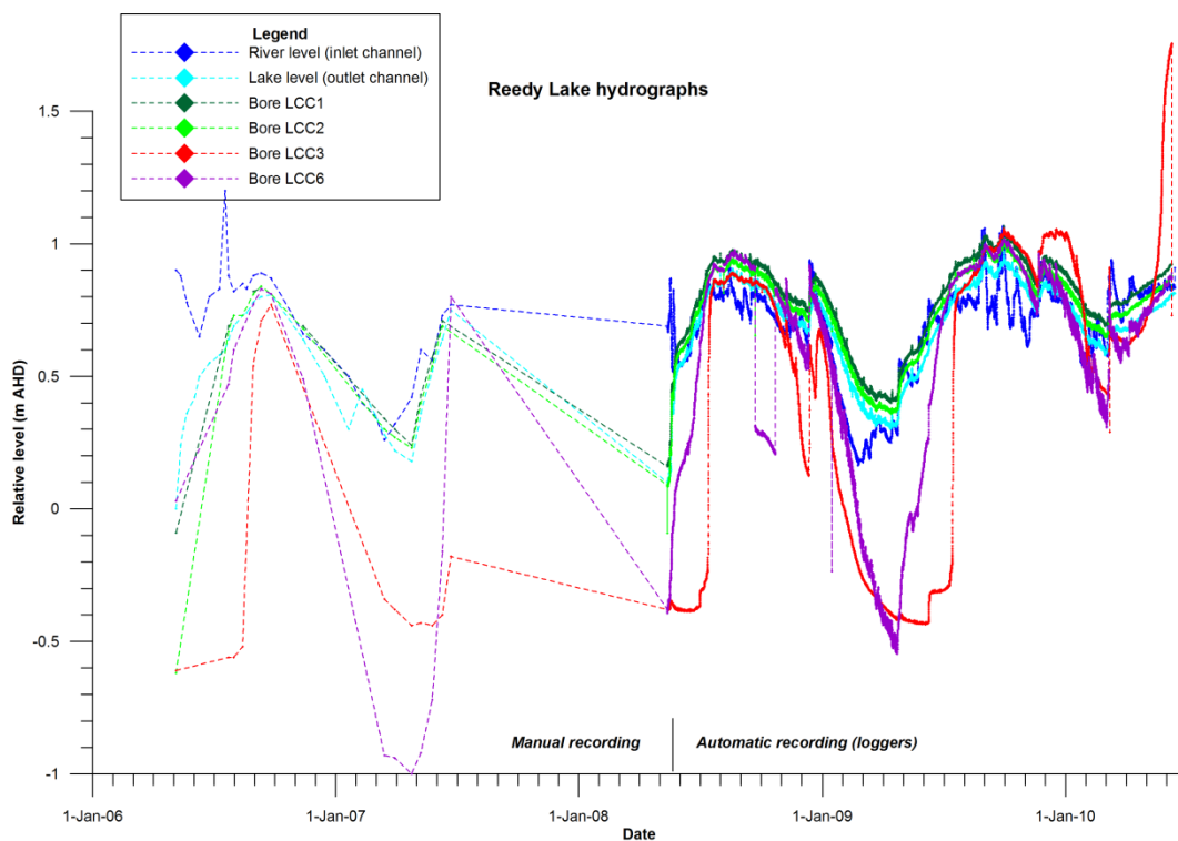
Figure 4: Response of Reedy Lake bores to river levels (raw data).
