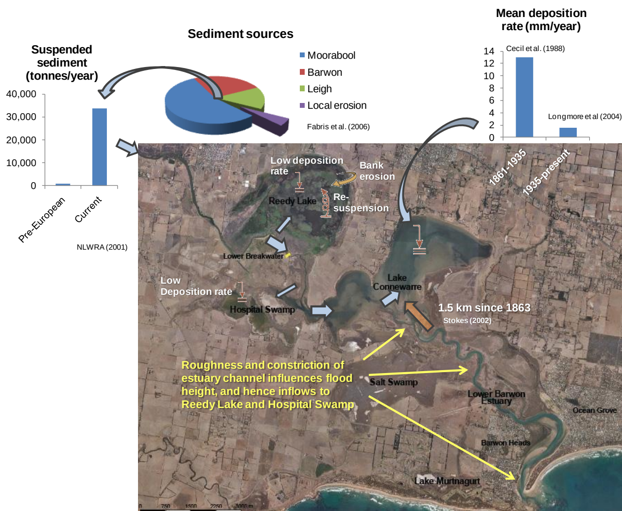
Figure 6: Conceptual model of the main geomorphological processes over the management time-scale.
