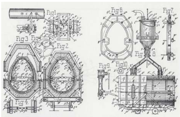
Stone & Siddeley's Patent concrete castings, 15.3.1912. Source: Willingham, 'Ovoid Sewer Aqueduct', 1991.
