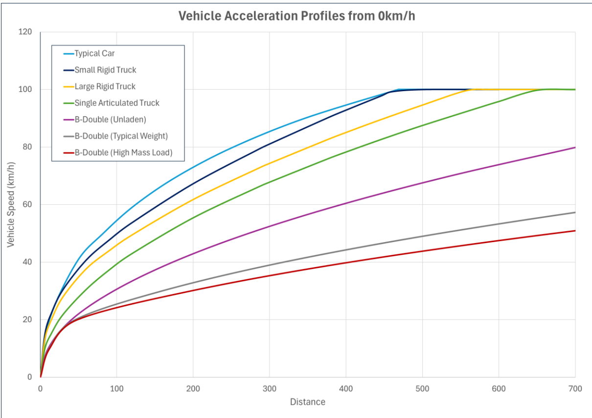
Figure 67: Typical Vehicle Acceleration Profiles from 0km/h
