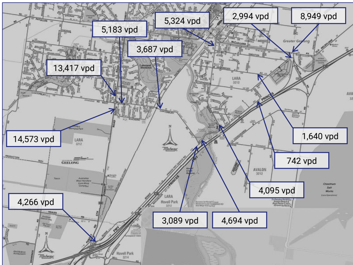
Figure 66: Post Development (including Sports Precinct) Traffic Volumes – Weekday Daily Average (Two-Way Volumes)
