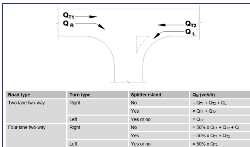
Figure 57: Calculation of Relevant Values (Figure 3.26, Austroads)
