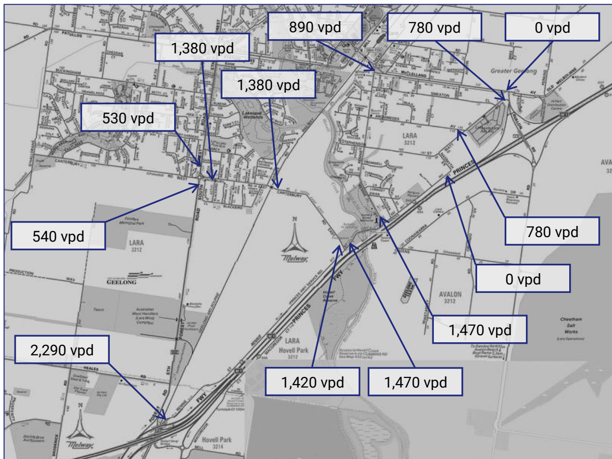
Figure 55: Site Generated Traffic Volumes - Weekday Daily Average (Two-Way Volumes)
