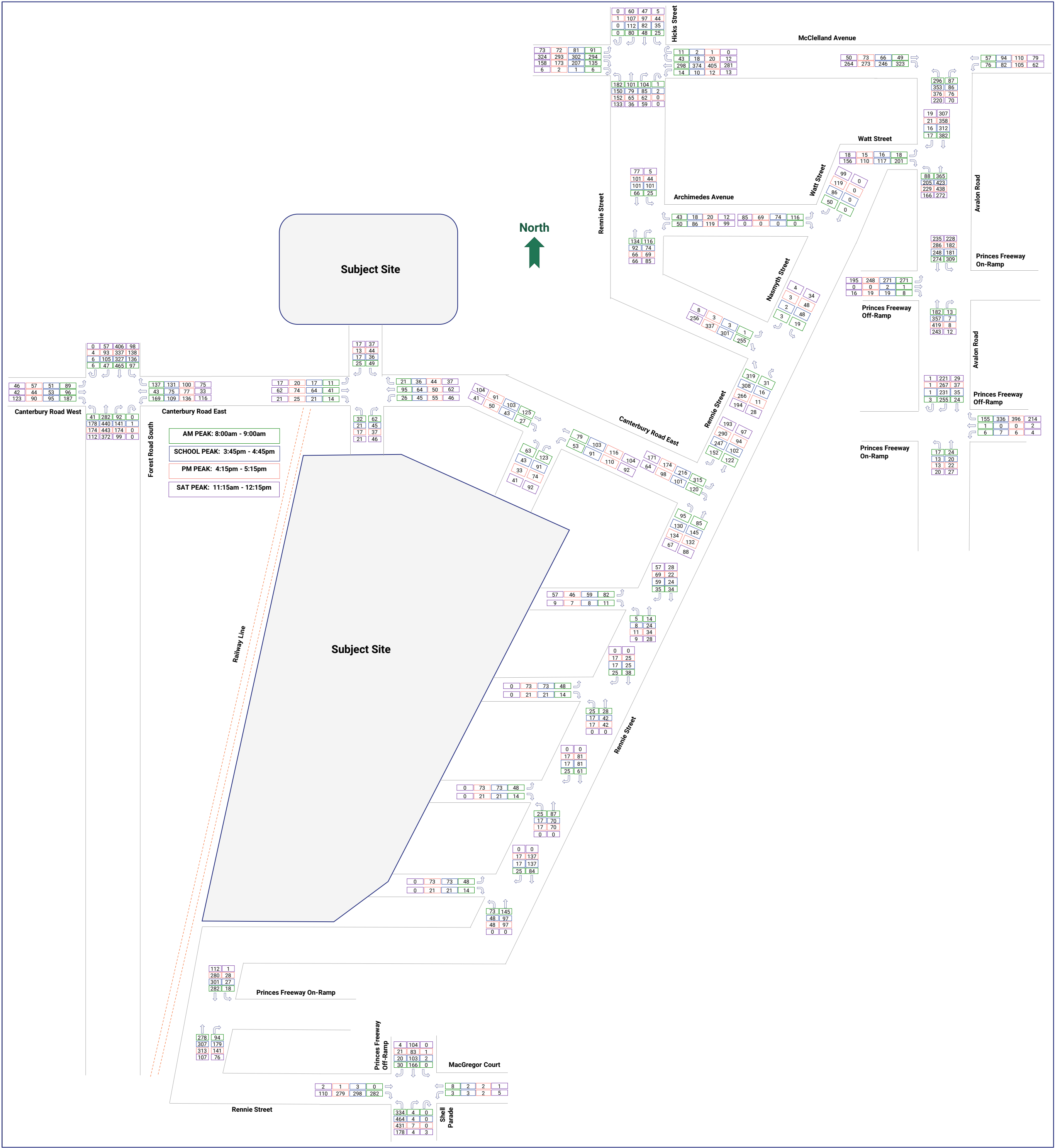
Figure 75: Post-Development Traffic Volumes with Northern Land Parcel Developed
