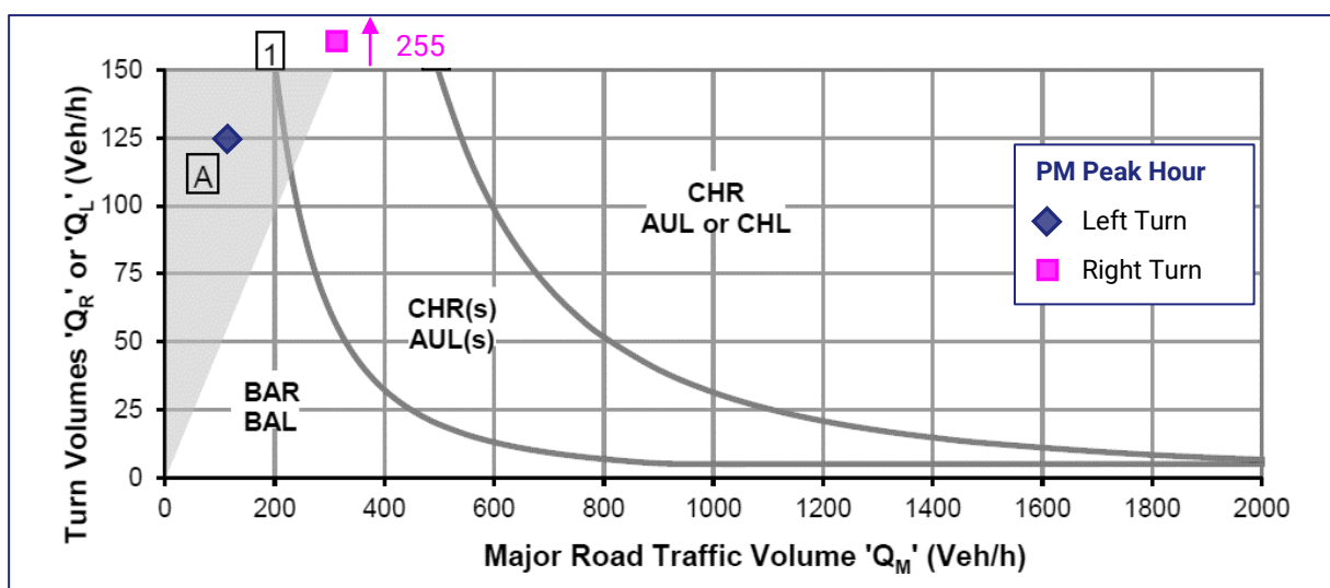
Figure 58: Left and Right Turn Warrants - Canterbury Road East/Rennie Street Intersection
