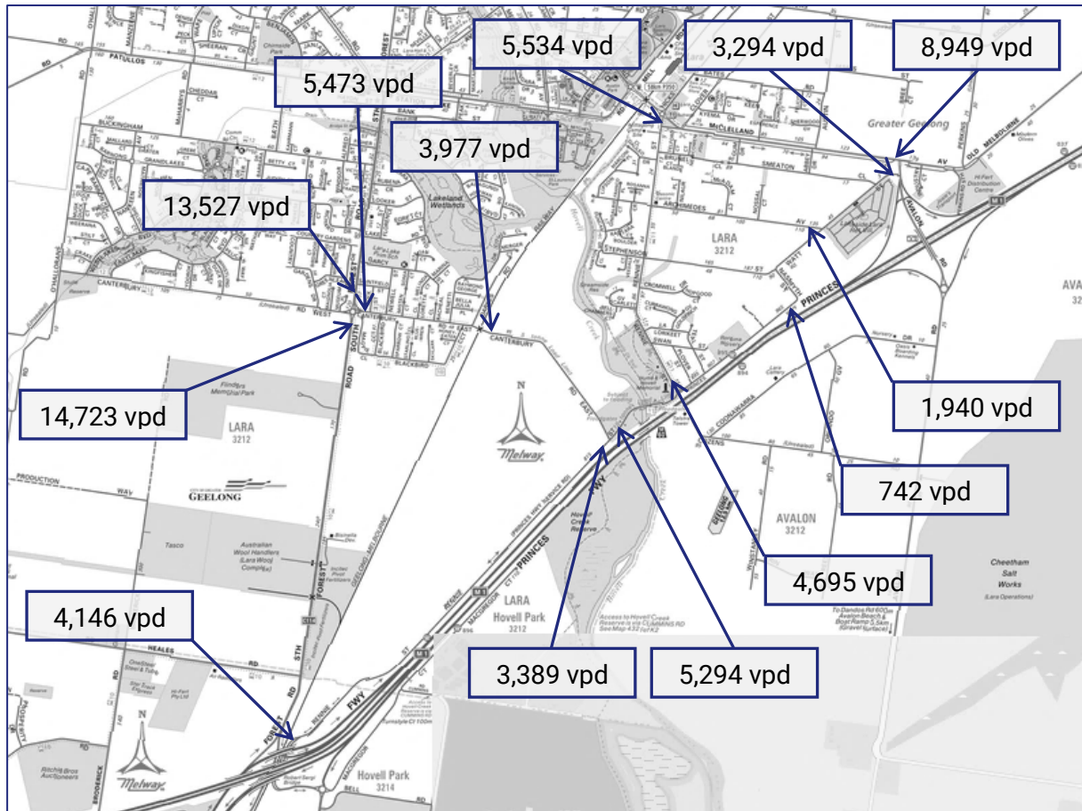
Figure 87: 7-Day Tube Count Results – Weekday Daily Average Two-Way Volumes (February, 2026)
