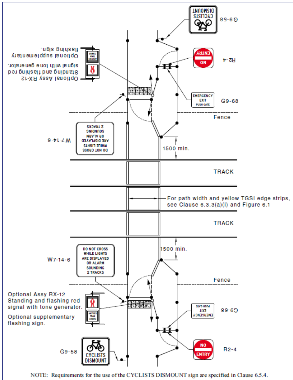
Figure 69: Active Gated Control Example (Figure F6, AS1742.7: 2016)
