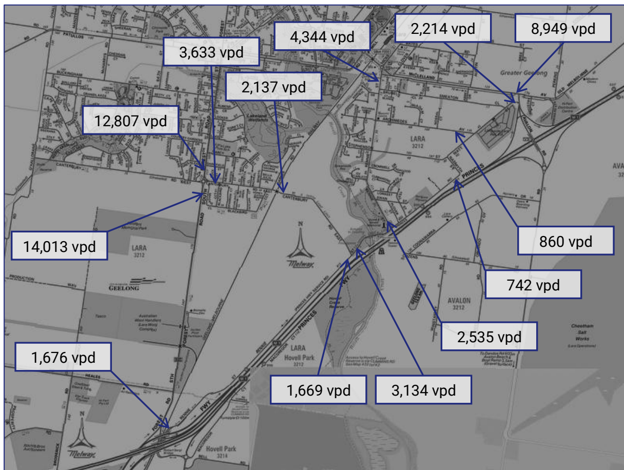
Figure 24: 7-Day Tube Count Results – Weekday Daily Average Two-Way Volumes (February, 2026)
